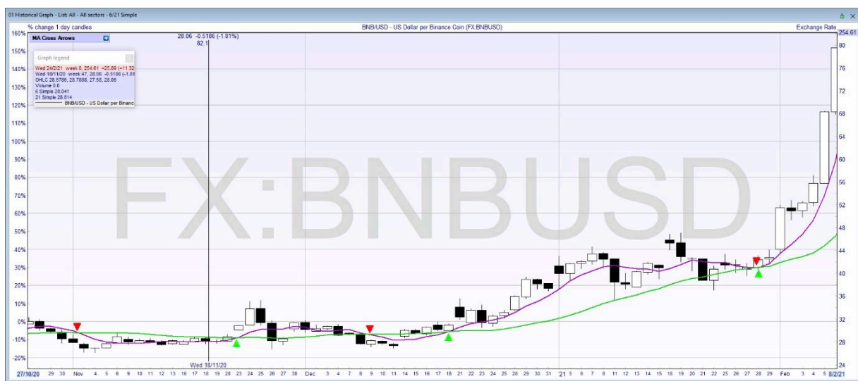
Figure 15 . Cross-over between a 6-day and a 21-day moving average
