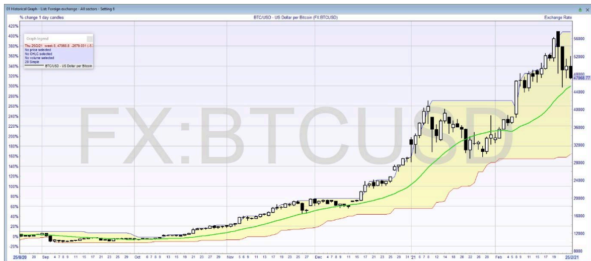
Figure 17 . A 20-day Donchian channel and a 20-day simple moving average
